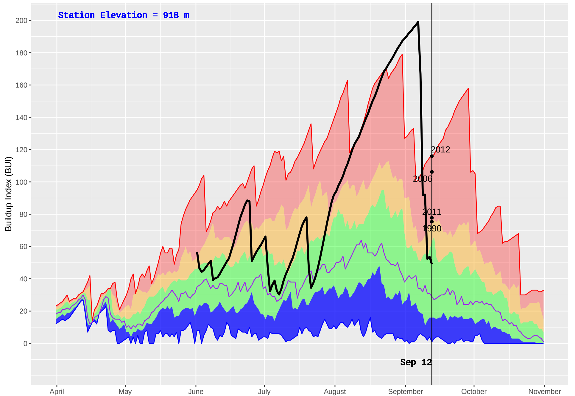
AUGIER LAKE (167) : Historical (1984–2016) and Current (2018) Daily Buildup Index (BUI)
